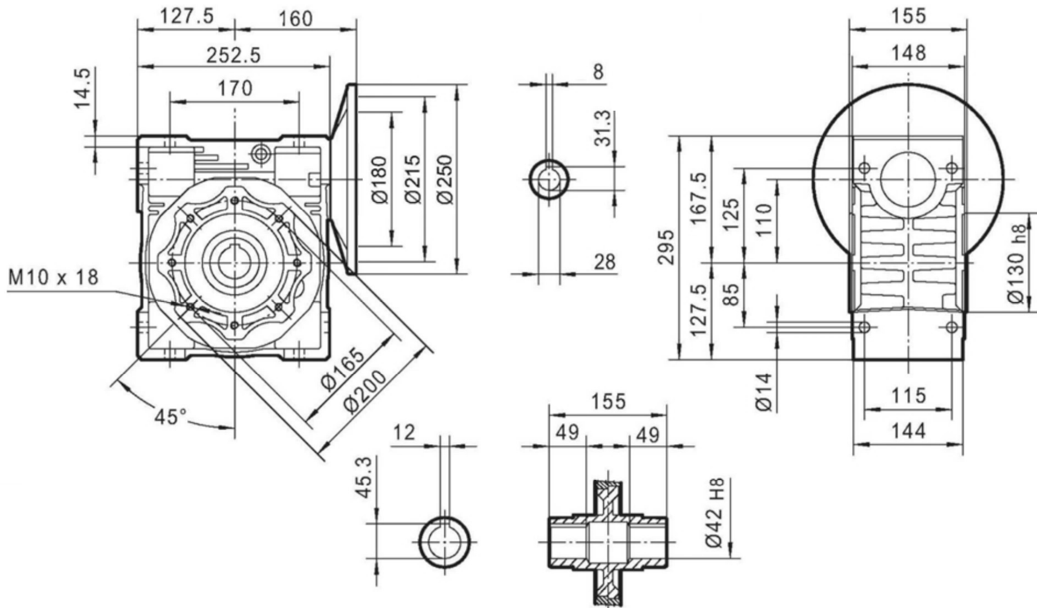
PMRV 110 100/112B5
