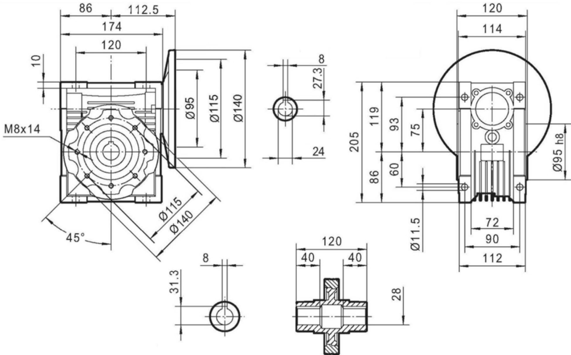
PMRV 075 90B14
